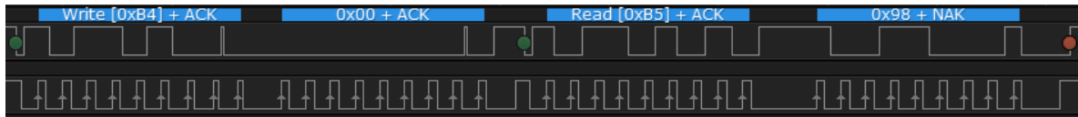
Figure 6: I 2 C Read Transaction To STATUS Register
