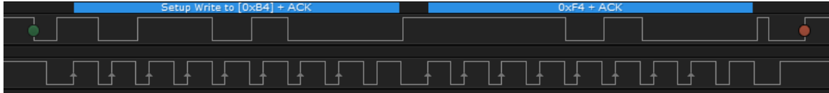
Figure 8: APP_START Interface
